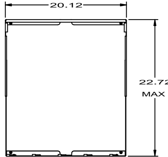
EXPANDED POSITION OCCUPIES 12RU WITH 11 USABLE RACK UNITS
