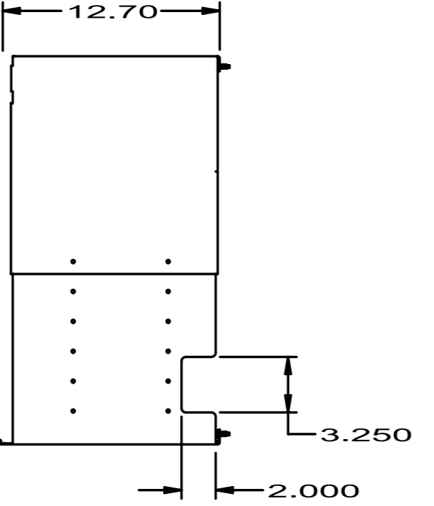
OVER 8RU CABLE ACCESS HOLE IS AVAILABLE LEFT & RIGHT SIDE
